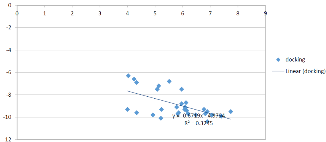
Figure 5: The coefficient of correlation of ( IC_{50} ) methionyl-tRNA synthetases
